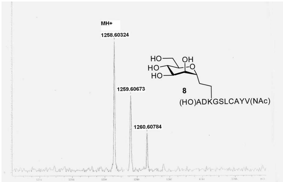
Figure 1: Mass spectra of glycopeptide 8 . Calculated mass = 1258.57512 Da, observed mass = 1258.60324 Da.
