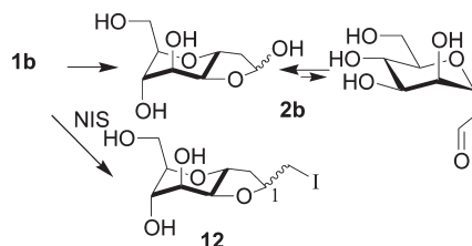
Scheme 3: Conformational change for mannoside derivatives.
