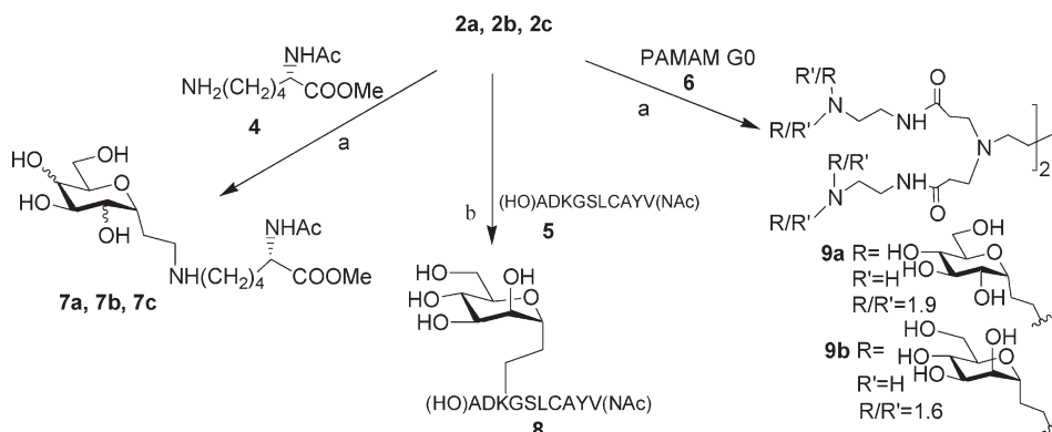
Scheme 4: Synthesis of derivatives 7 , 8 , and 9 by reductive amination. Reagents and conditions: a) MeOH, NaCNBH 3 , AcOH; b) MeOH/H 2 O, NaCNBH 3 , AcOH.
