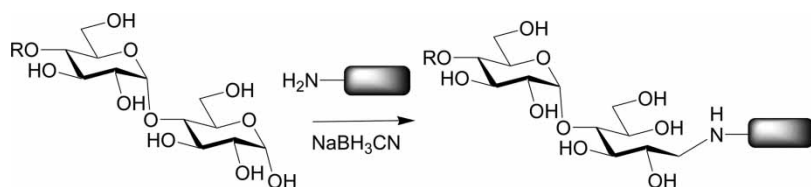
Scheme 1: Glycoconjugation by reductive amination.
