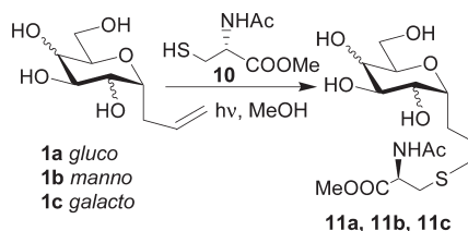
Scheme 5: Chemoselective synthesis of cysteine conjugates 11 .
