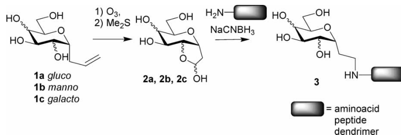
Scheme 2: Synthesis of bicyclic hemiacetals 2 and their conjugation.
