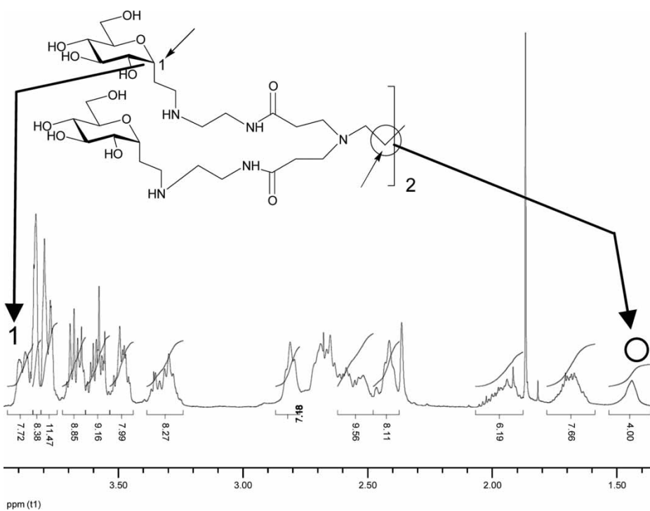
Figure 2: 1 H NMR of signal integration of glucodendrimer 9a .
